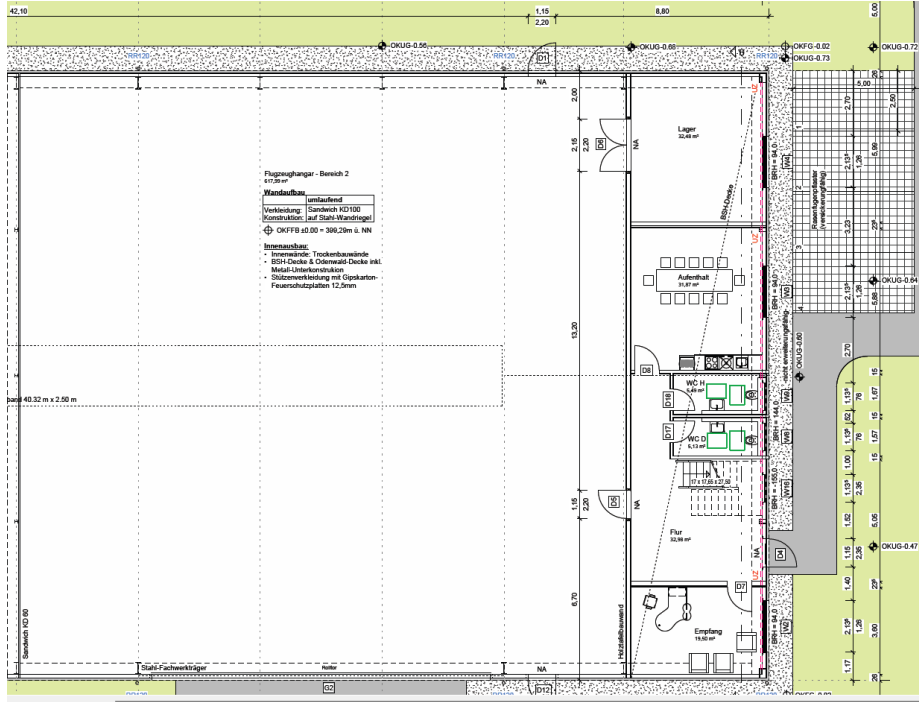
EG (Hangar + Räume)
